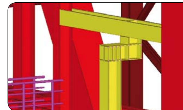
A small section of the overall Wai GaoQiao model. The existing construction (imported as an SDNF file) is shown in red, the extension planning with Tekla Structures in yellow. The object in question is an additional pipeline support.
