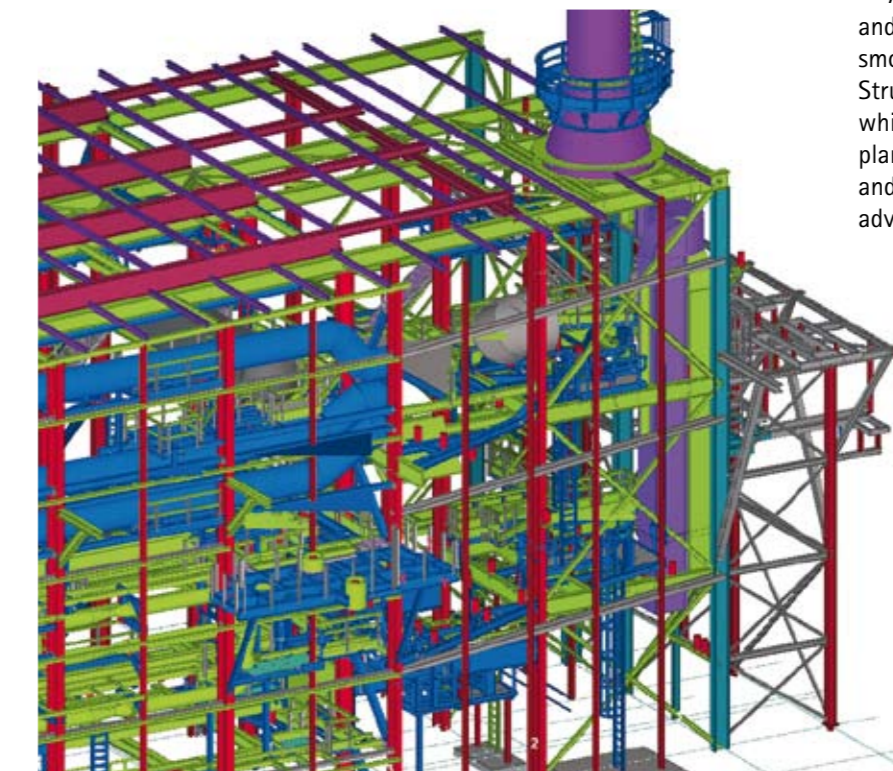
A small section of the overall Wai GaoQiao model. The existing construction (imported as an SDNF file) is shown in red, the extension planning with Tekla Structures in yellow. The object in question is an additional pipeline support.
